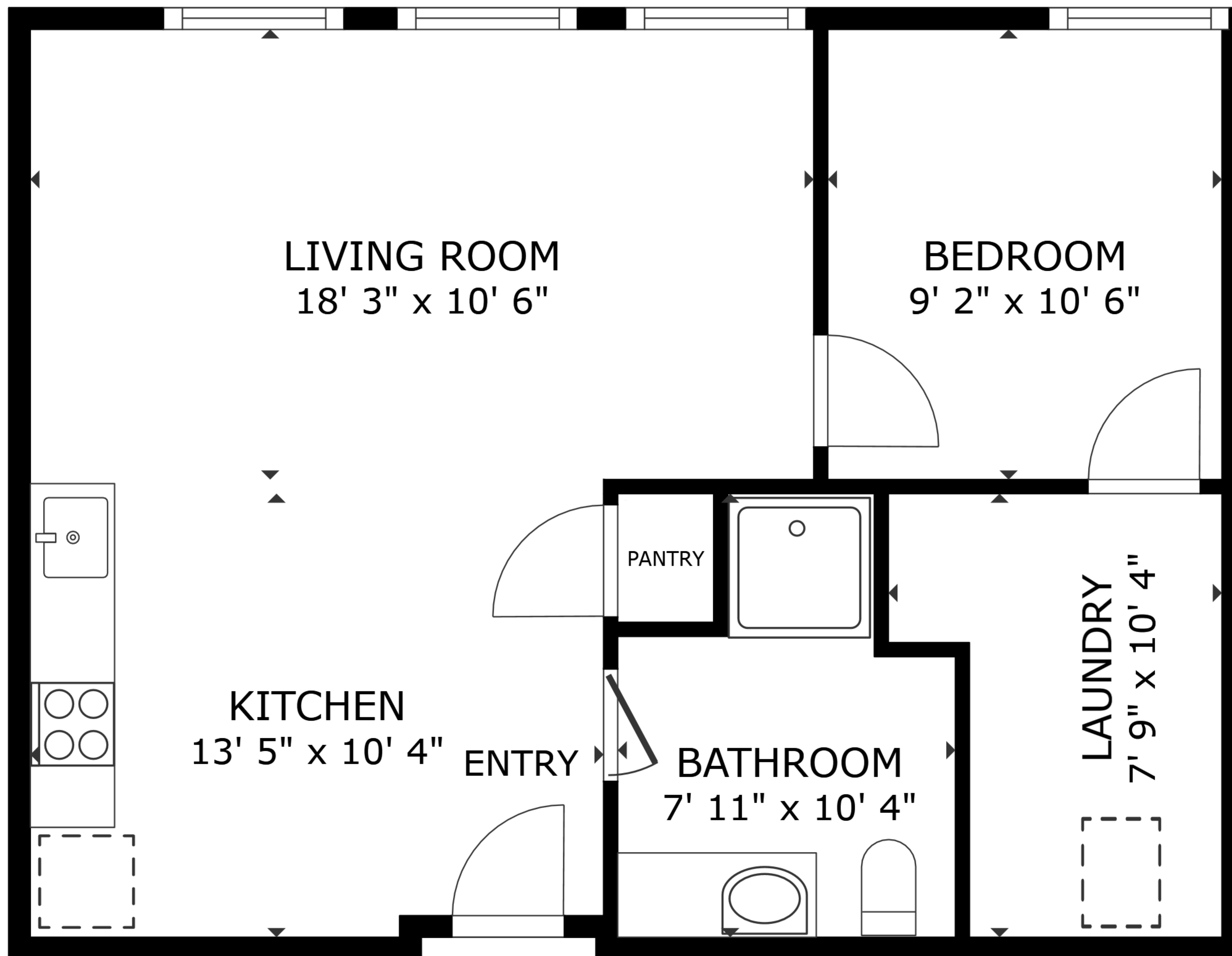
FLOOR PLAN
