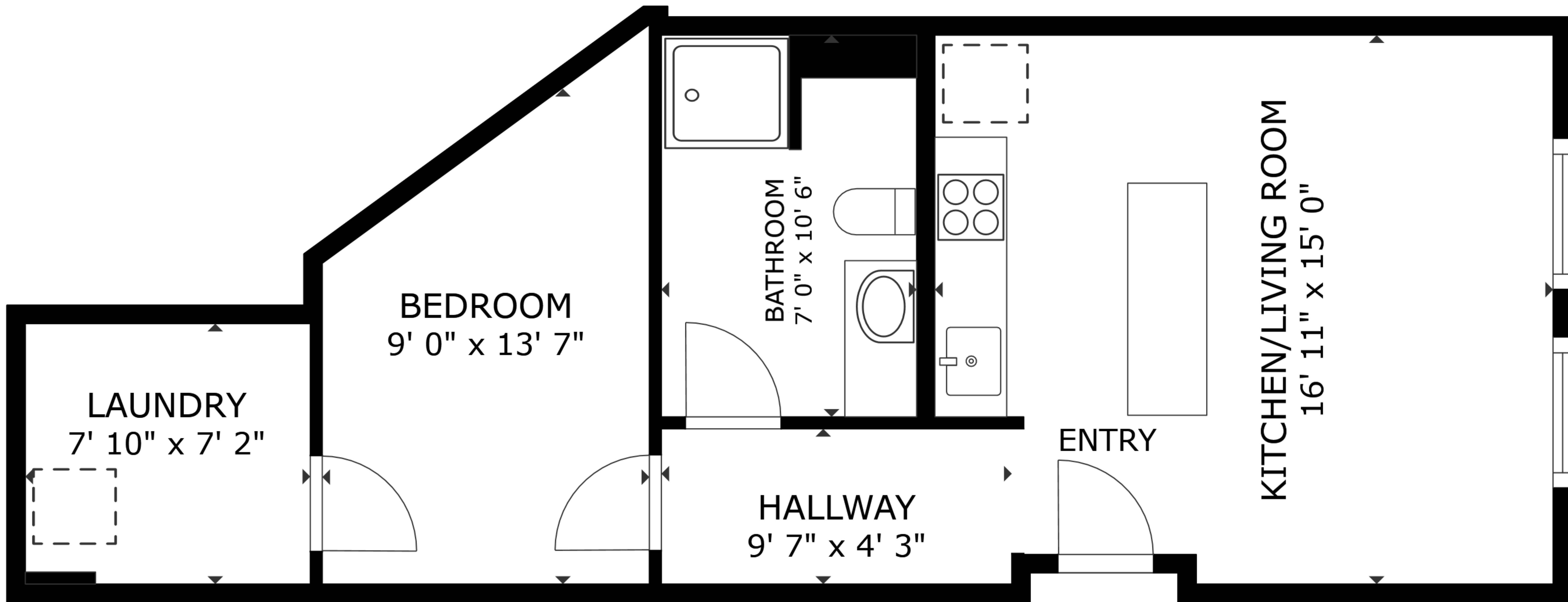
FLOOR PLAN
