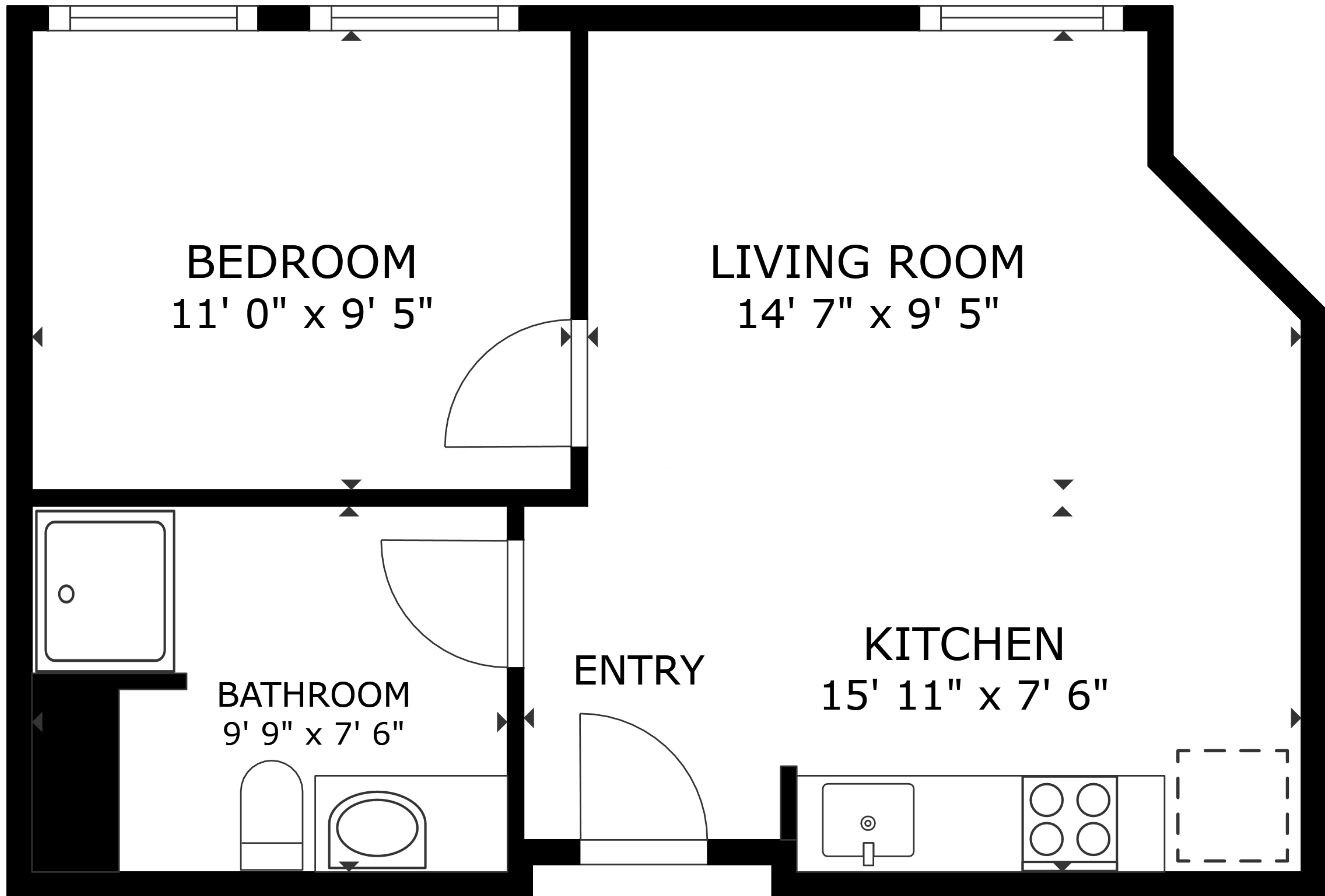
FLOOR PLAN
